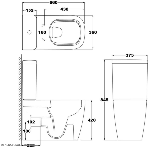
DIMENSIONAL DRAWING
