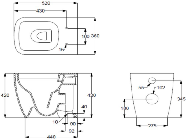
DIMENSIONAL DRAWING
