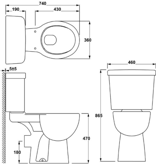
DIMENSIONAL DRAWING
