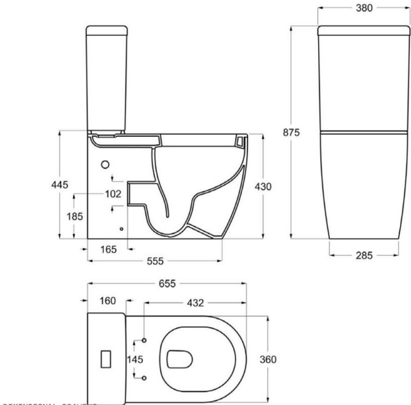
DIMENSIONAL DRAWING
