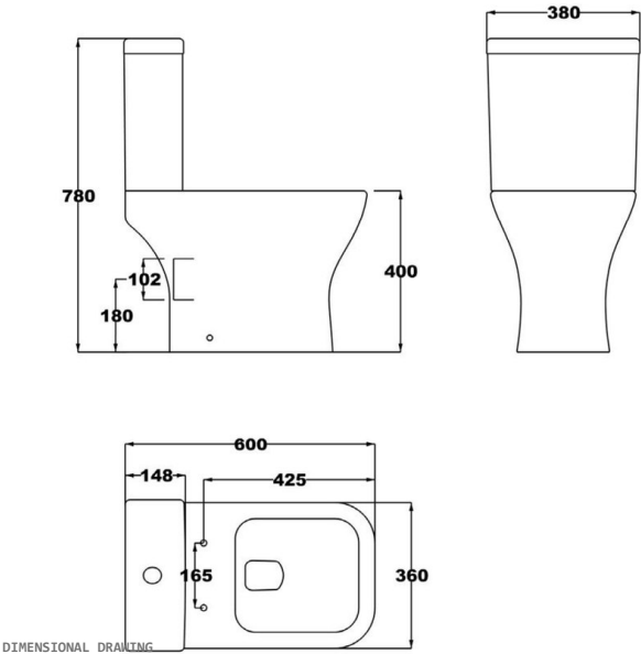
DIMENSIONAL DRAWING
