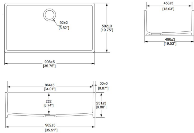
DIMENSIONAL DRAWING
