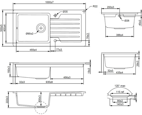
DIMENSIONAL DRAWING
