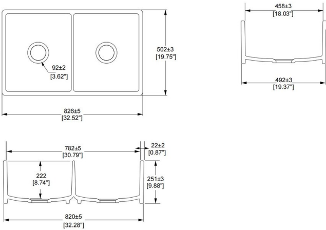
DIMENSIONAL DRAWING
