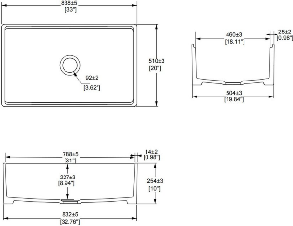
DIMENSIONAL DRAWING
