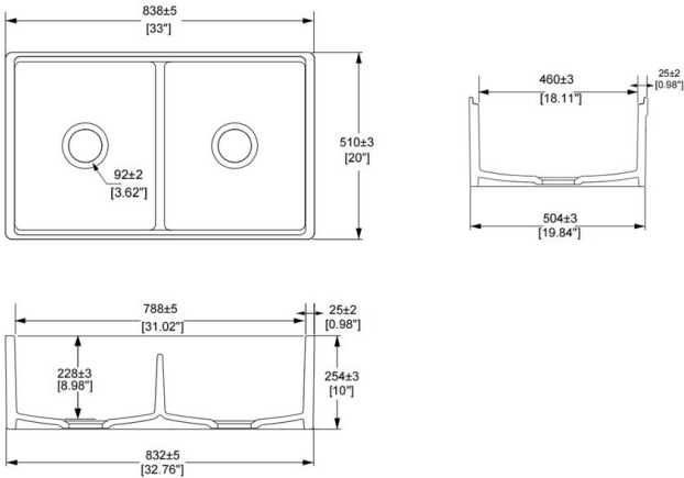
DIMENSIONAL DRAWING
