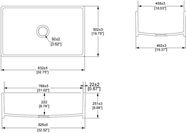
DIMENSIONAL DRAWING
