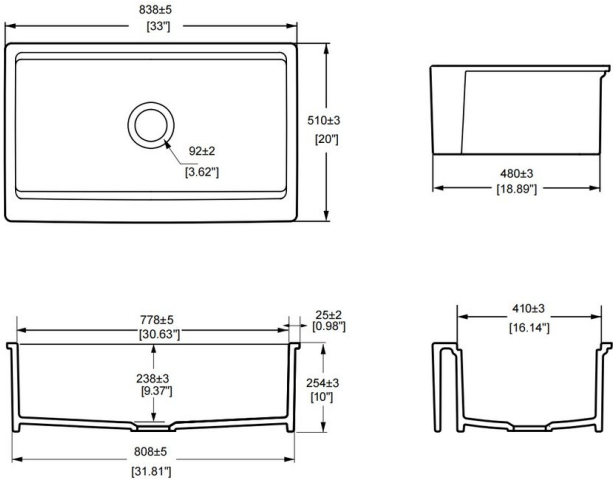
DIMENSIONAL DRAWING
