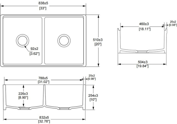
DIMENSIONAL DRAWING
