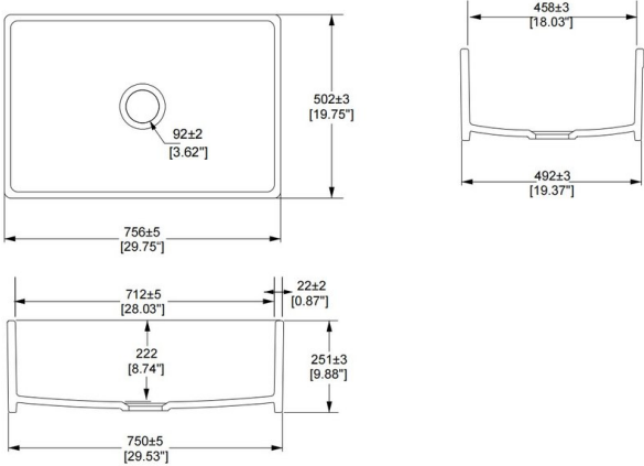
DIMENSIONAL DRAWING
