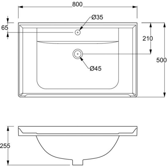
DIMENSIONAL DRAWING
